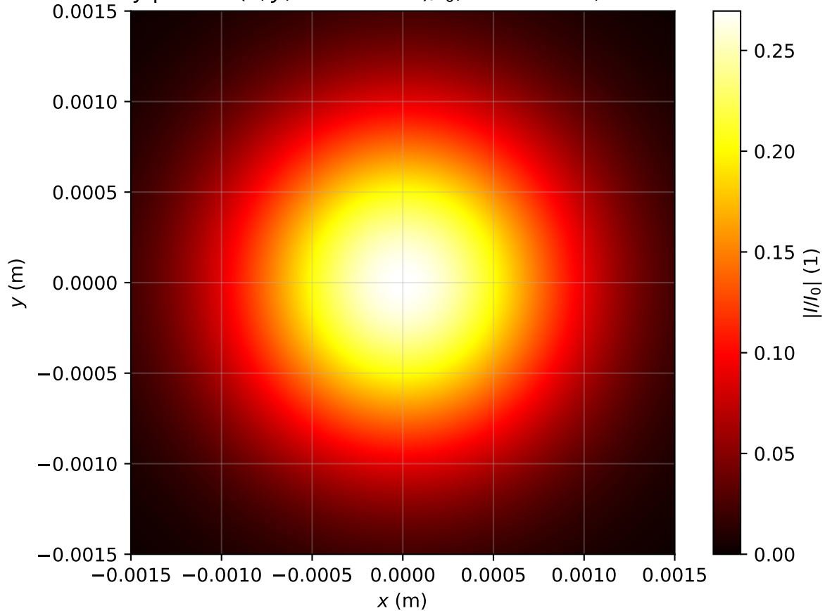
Intensity profile I(x, y, z = 3.503m)/I_0 , P_{in}=0.1P_{cr} , artificial time
